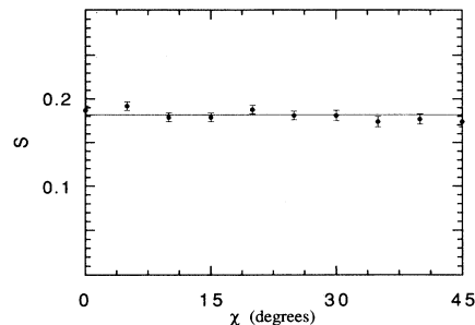
FIG. 2. Experimental results for the parameter S and its standard deviation in the Bell inequality for various settings \chi of the quarter-wave plates.
