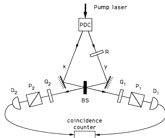
FIG. 1. Outline of the experiment for testing local realism by polarization-correlation measurements.
